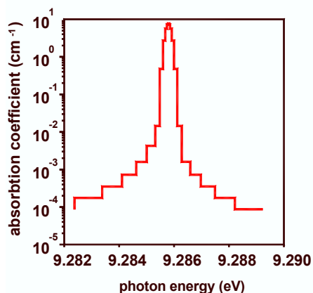
Fig. 3. CII ion line corresponding to the transition 2s^2(1S)2p^2-2p^3 .
