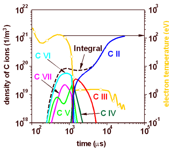
Fig. 2. Time dependence of carbon plasma temperature and the densities of different carbon ions species at the separatrix, 3.8 m from the outer divertor.
