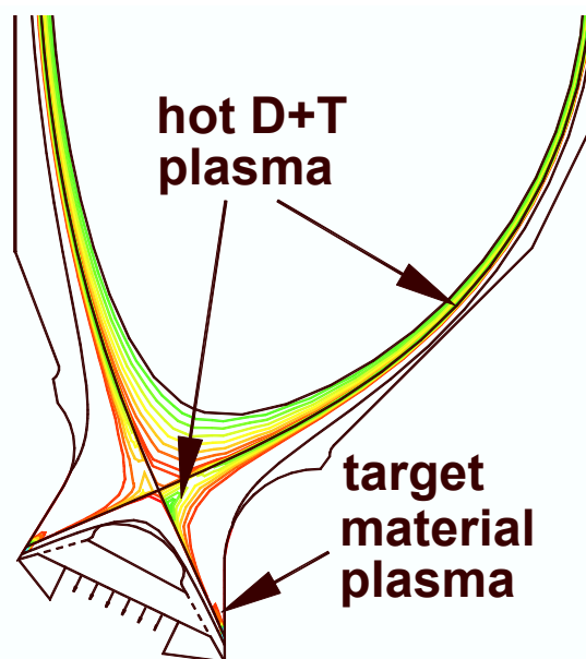
Fig. 1. General view of ITER poloidal cross-section used in FOREV simulations
