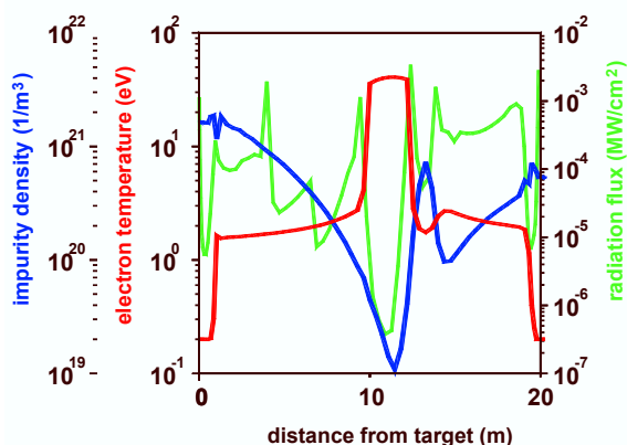
Fig. 4. Temperature, density and radiation flux from the carbon plasma along the separatrix
